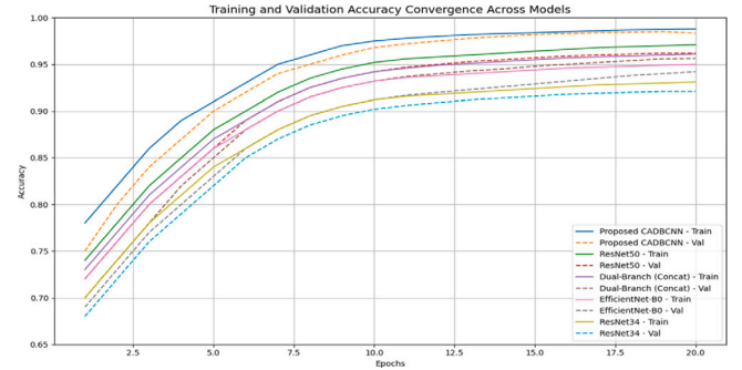
Fig. 8. Training and Validation Accuracy.
