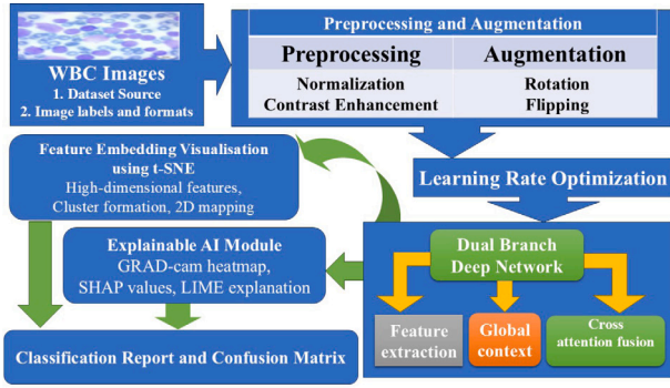
Fig. 1. Dual-Branch Deep Learning Pipeline for Explainable Leukemia Image Classification.
