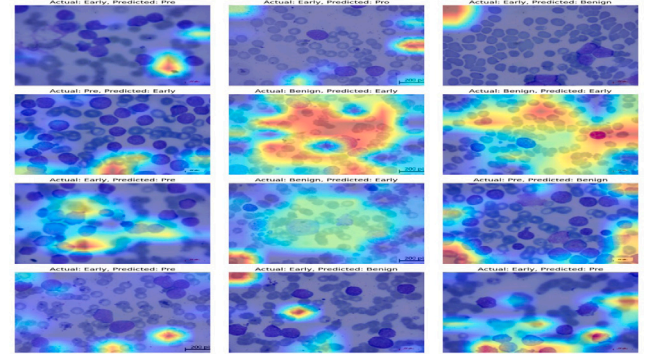
Fig. 5. Grad-CAM Heatmaps (for sample 1 to 12)
