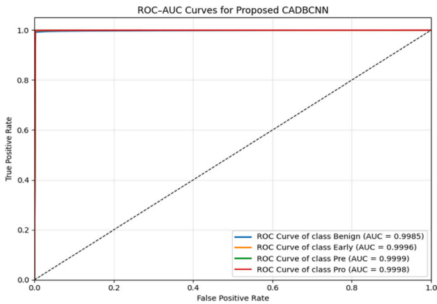
Fig. 7. ROC-AUC Curves for proposed CADBCNN.
