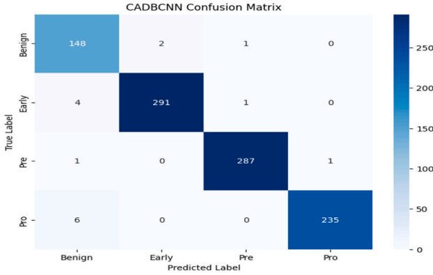
Fig. 6. Confusion Matrix of Proposed Model.
